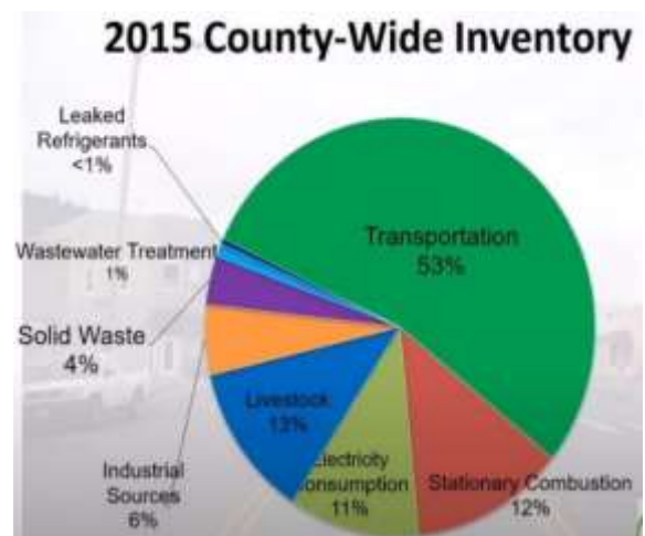
Figure Climate-3. 2015 Humboldt County Greenhouse Gas Emissions (Draft County CAP)
