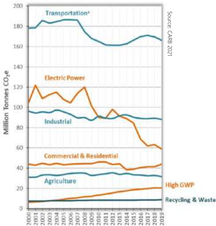
Figure Climate-4. Trends in California GHG Emissions, 2000-2019
