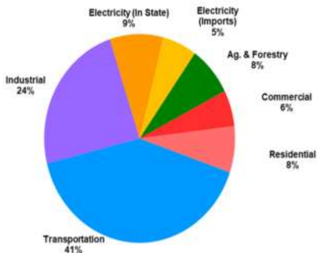
Figure Climate-2. Sources of California Greenhouse Gas Emissions in 2019
