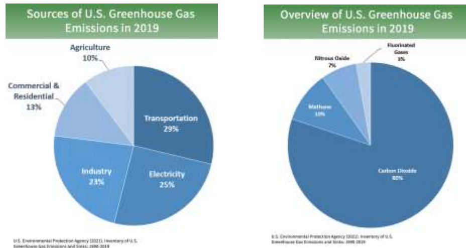
Figure Climate-1. U.S. Greenhouse Gas Emission in 2019
