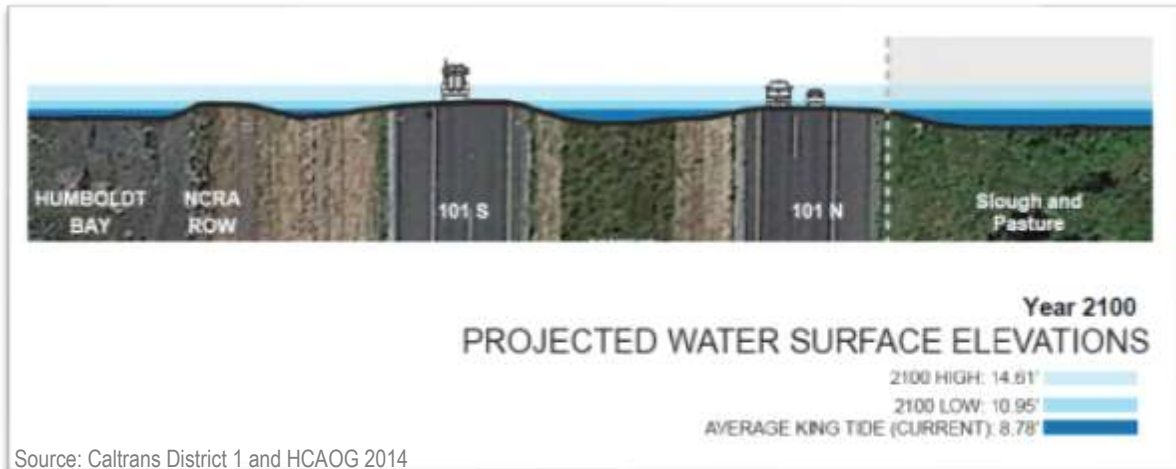
Figure Climate-5. Highway 101 Vulnerability to Sea-Level Rise Along Humboldt Bay Water heights predicted for year 2100 under the high GHG emission scenario and the annual average King tide.
