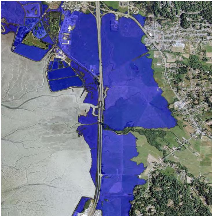
Figure Climate-8. North segment, upper Arcata Bay Reach projected inundation 2015–2050
