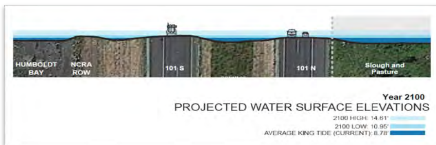
Figure Climate-5 . Highway 101 Vulnerability to Sea-Level Rise Along Humboldt
